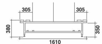
Depth of double-sided bench
