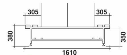
Depth of double-sided bench
