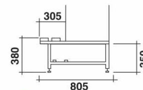
Depth of single-sided bench
